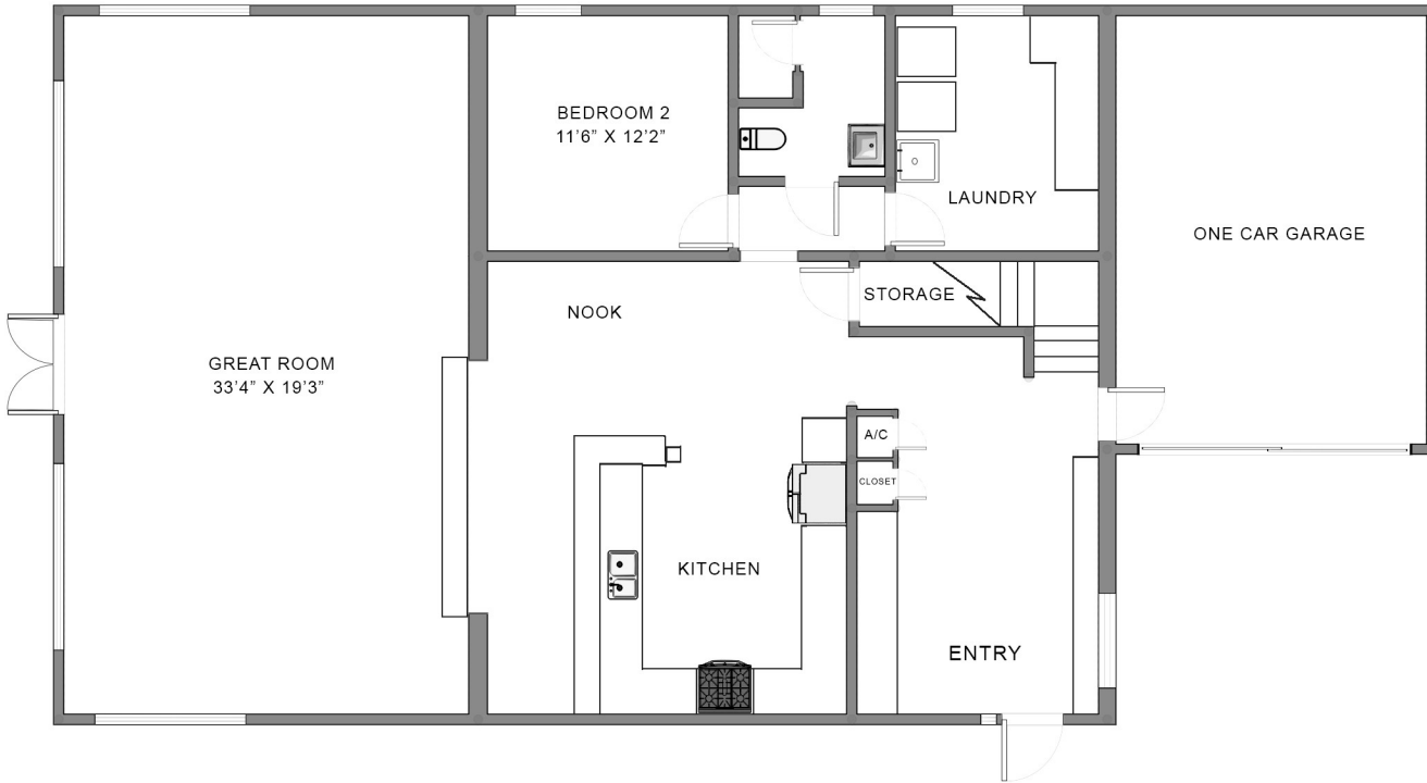
FIRST FLOOR
